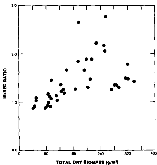
(c) r^2 = 0.32
