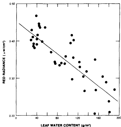
(a) 0.63\text{--}0.69\ \mu\text{m} r^2 = 0.70 Y = 0.45534 - 0.00108 \cdot X
