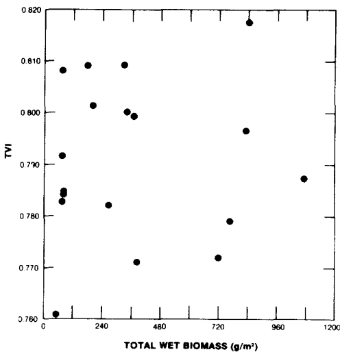
(i) r^2 = 0.00
