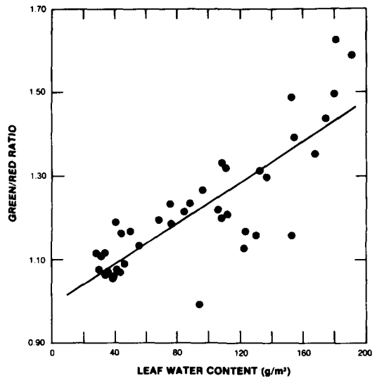
(f) r^2=0.67 Y=0.9933+0.0024 \cdot X September data
