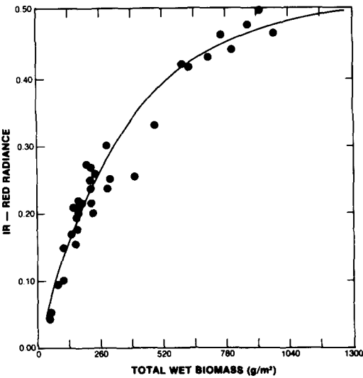
(e) r^2=0.89 Y=0.51-\exp(-0.6713-0.0028\cdot X)
