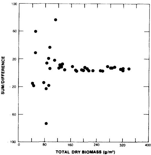
(h) r^2 = 0.00
