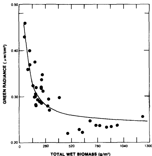
(a) 0.52\text{--}0.60\text{ }\mu\text{m} r^2 = 0.79 Y = 0.237 + 12.129/X June data
