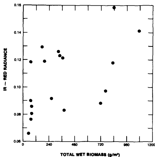
(e) r^2=0.28
