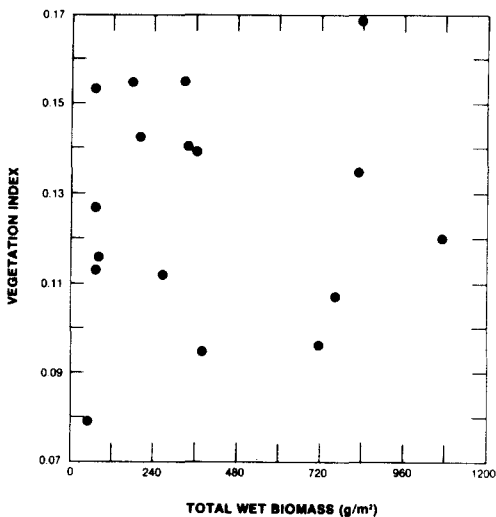
(g) r^2 = 0.00
