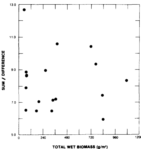
(h) r^2 = 0.01
