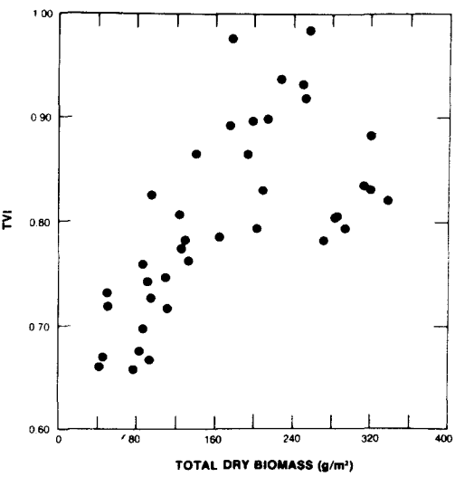
(i) r^2 = 0.44
