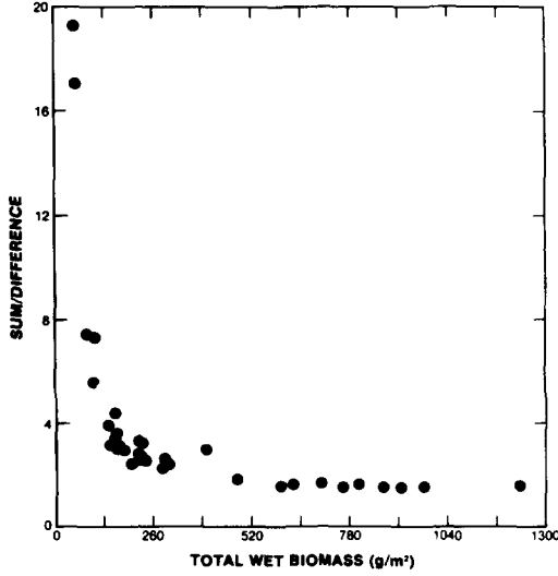
(h) r^2=0.94
