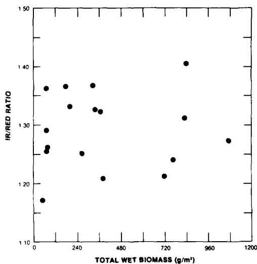
(c) r^2=0.00
