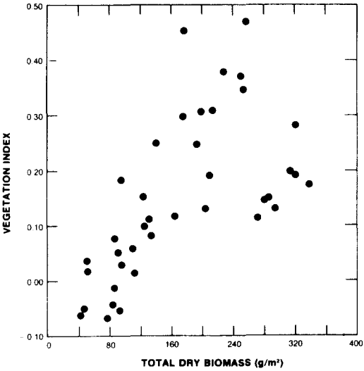
(g) r^2 = 0.42
