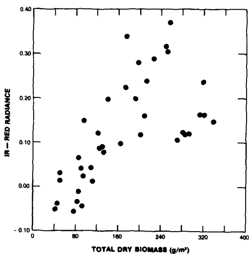
(e) r^2 = 0.45
