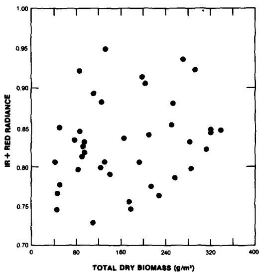
(f) r^2 = 0.05
