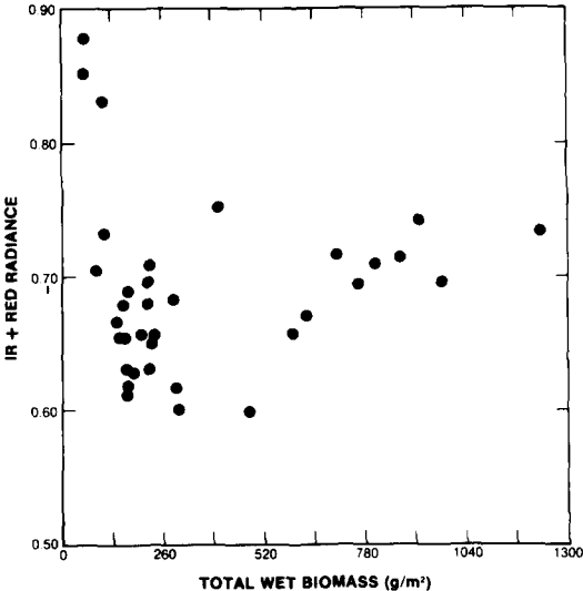
(f) r^2=0.00
