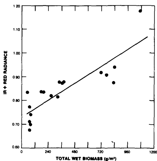
(f) r^2=0.72 Y = 0.73444 + 0.00029 \cdot X
