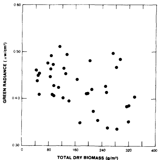
(b) 0.52\text{--}0.60\text{ }\mu\text{m} r^2 = 0.14 September data
