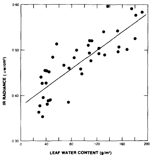
(b) 0.75\text{--}0.80\ \mu\text{m} r^2 = 0.68 Y = 0.37860 + 0.00102 \cdot X
