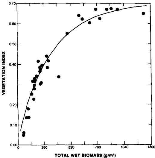
(g) r^2=0.89 Y=0.70-\exp(-0.4207-0.0030\cdot X)
