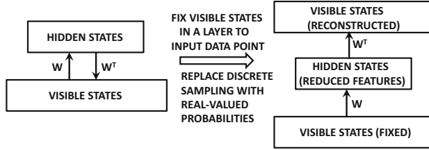
Figure 6.4: Using trained RBM to approximate trained autoencoder
