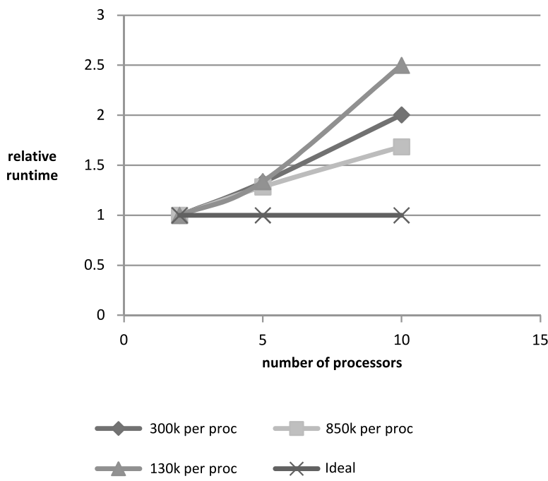
Figure 13.6 Scale-up of PMCRI Using Relative Runtimes
