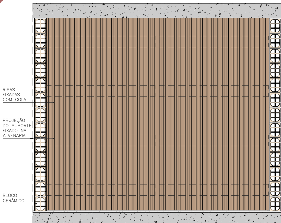
VISTA FRONTAL
