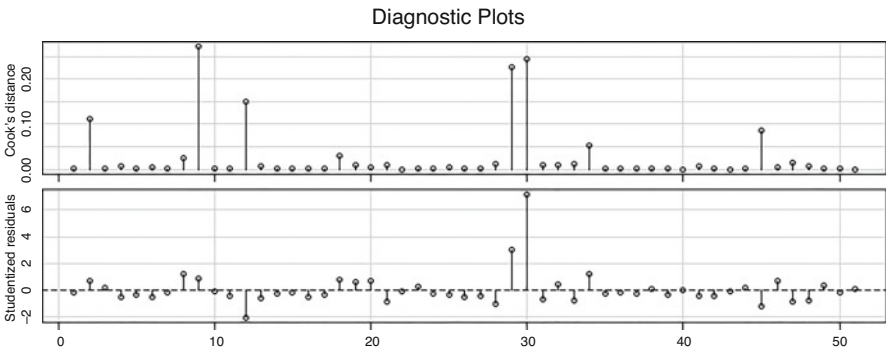
Fig. 7.10 Index plots for cigarette consumption model in Table 7.7
