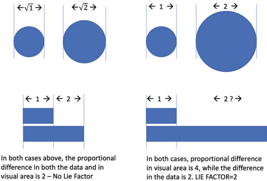
Fig. 5.21 Lie factors in proportional differences
