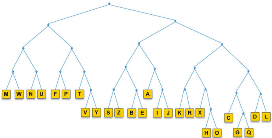
Fig. 16.18 A binary hierarchical classifier for a 26-class classification problem
