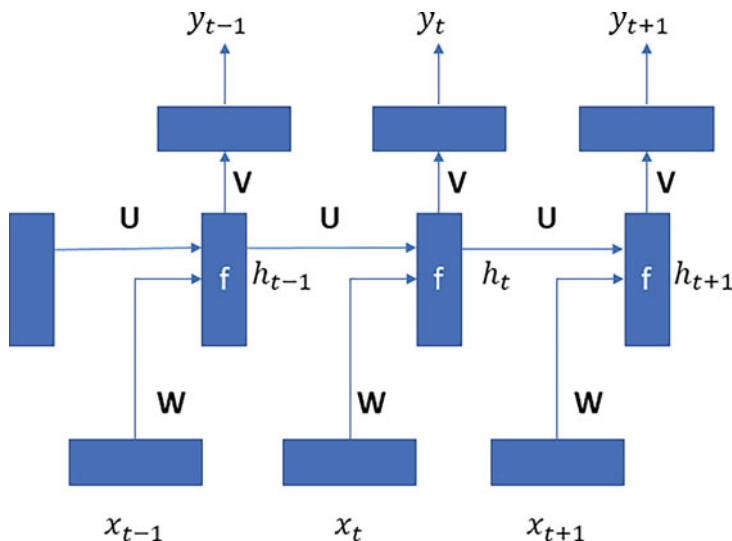
Fig. 17.7 Basic RNN architecture
